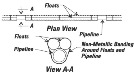
Figure 6 Flotation on the Surface
