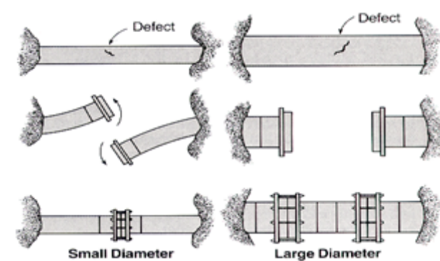
Figure 23 Repair Connections
