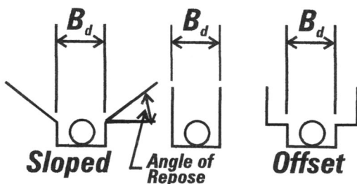
Figure 25 Trench Width
