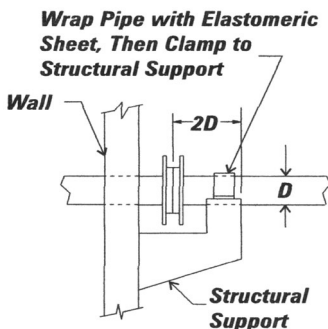
Figure 31 Protecting Connections to Flanges and Fittings
