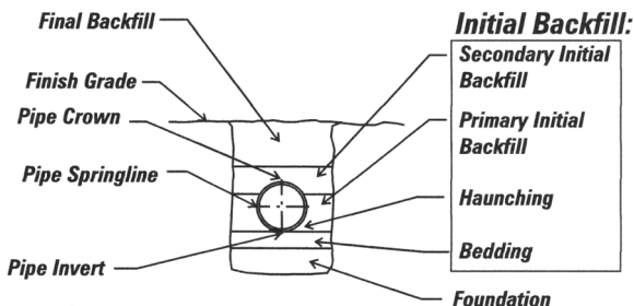
Figure 24 Embedment Terminologies
