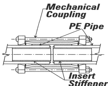
Figure 17 Mechanical Coupling with Insert Stiffeners
