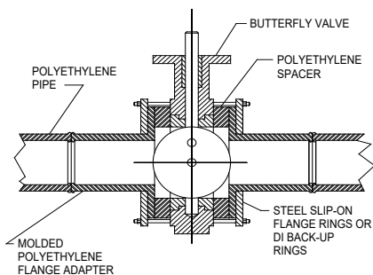
Figure 16 Butterfly Valve Connections
