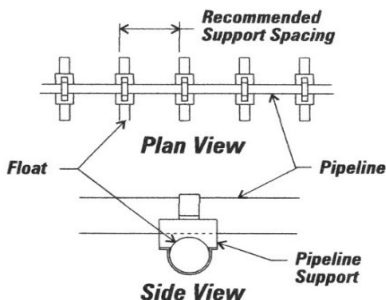
Figure 6 Flotation on the Surface
