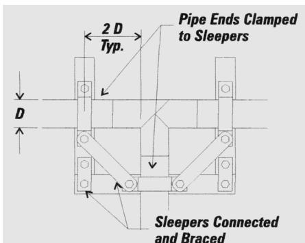
Figure 39 Surface Tee Bending Protection
