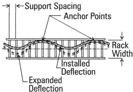
Figure 41 Pipe Rack, Side Anchored
