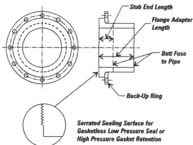
Figure 11 Flange Adapter and Back-Up Ring
