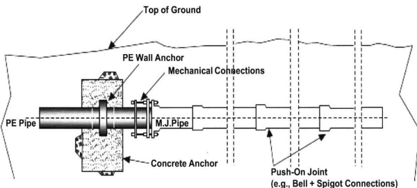
Figure 34 Pullout Prevention Technique #2
