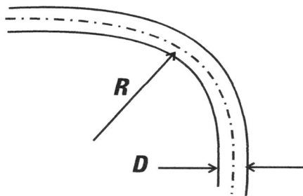
Figure 27 Bend Radius
