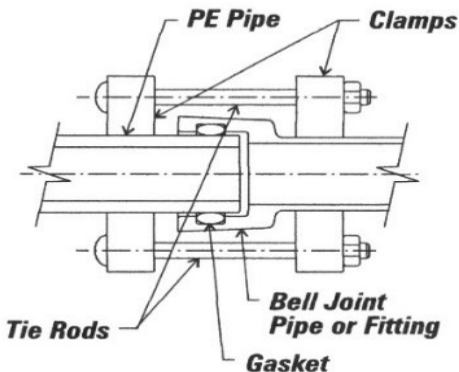
Figure 20 External Joint Restraint
