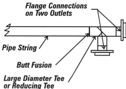
Figure 21 Large Diameter Tee Installations
