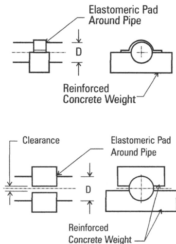
Figure 4 Concrete Ballast Weight
