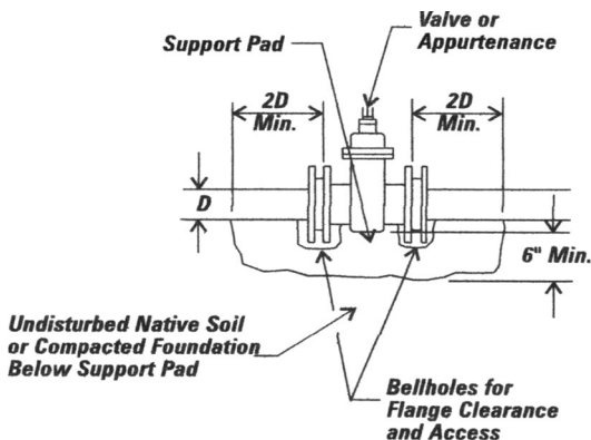
Figure 32 Appurtenance Support Pad
