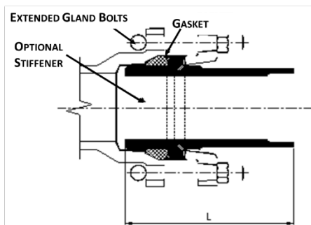
Figure 10 DriscoPlex® MJ Adapter with Optional Stiffener
