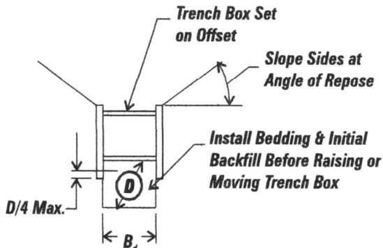
Figure 26 Trench Box Installations
