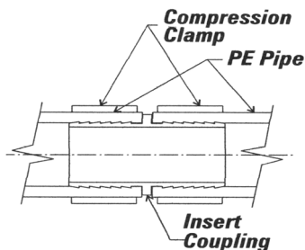
Figure 18 Insert Coupling
