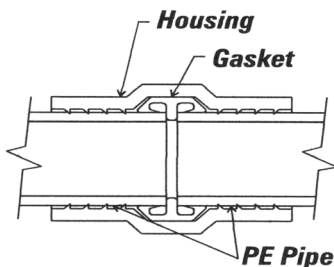
Figure 19 Partially Restrained Compression Coupling
