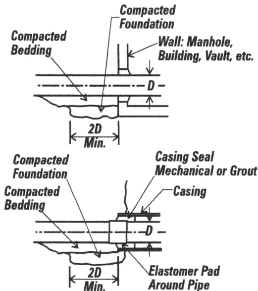
Figure 29 Controlling Shear and Bending Loads
