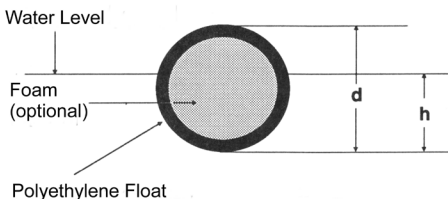
Figure 7 Float Submergence
