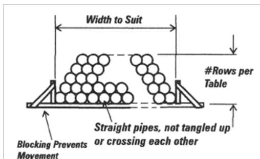
Figure 9 Loose Pipe Storage
