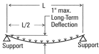
Figure 3 Support Spacing
