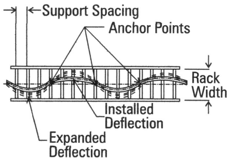
Figure 40 Pipe Rack, Center Anchored
