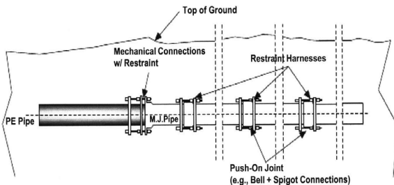
Figure 34 Pullout Prevention Technique #2
