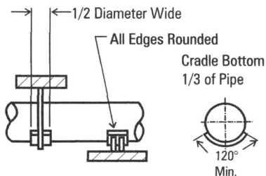
Figure 1 Pipeline Supports
