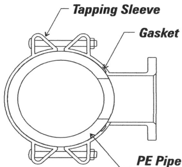
Figure 22 Tapping Sleeve
