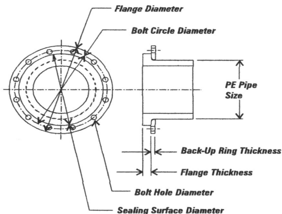
Figure 12 Flange Adapter and Back-Up Ring
