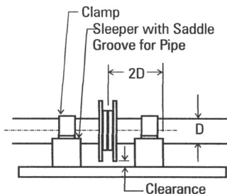
Figure 31 Protecting Connections to Flanges and Fittings
