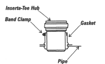
Figure 38 Inserta-Tee®
