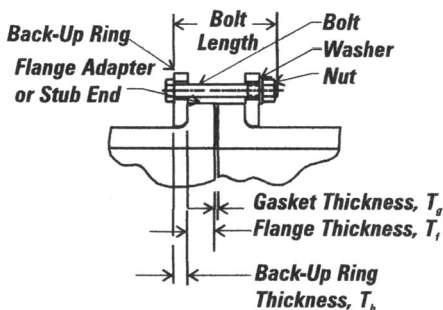
Figure 14 Flange Bolt Length
