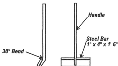
Figure 28 Haunch Tamping Tool
