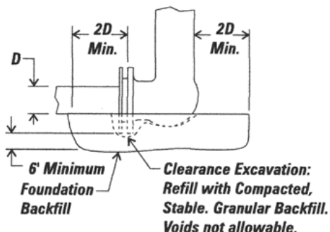
Figure 15 Buried Flange Connection Foundation
