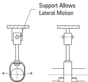
Figure 2 Pipeline Hanger
