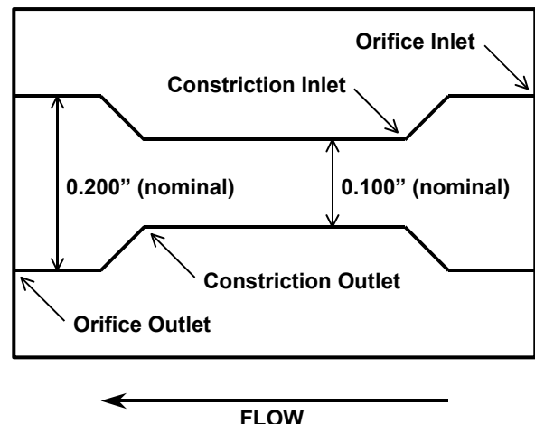
Figure 1. Wear Resistance Test Orifice
