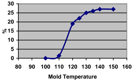
Figure 3. Crystallinity at various mold temperatures, as measured by XRD
