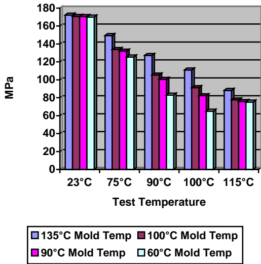
Figure 6. Tensile strength tested at elevated temperatures.
