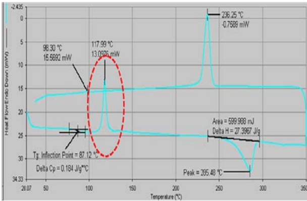
Figure 2. DSC of amorphous (cold molded) PPS part illustrating the Tc associated with crystallization in the oval.
