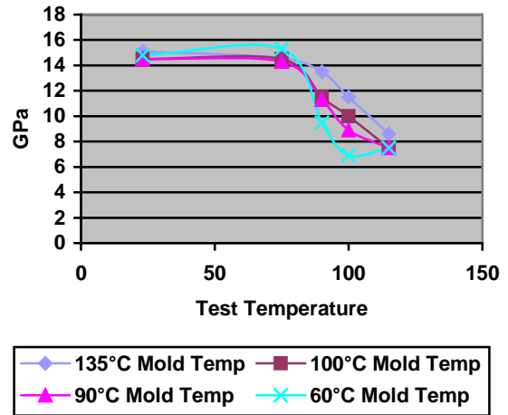
Figure 9. Tensile modulus tested at temperature, note the difference in hot and cold molded values at 100°C.
