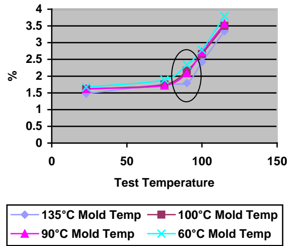
Figure 8. Tensile elongation tested at temperature, note the difference between hot and cold molded samples at 90°C in the circled area.
