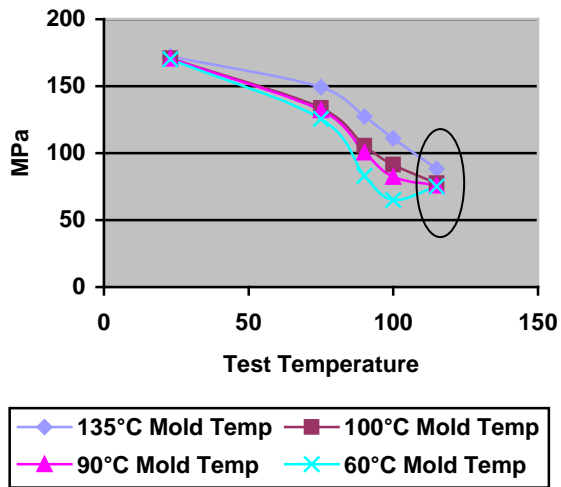
Figure 7. Tensile strength tested at temperature, note the convergence of the test results in the circled area, as the test temperature exceeds the T g and crystallization takes place.
