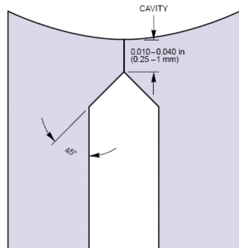
Figure 2 Typical Pinch-off Section
