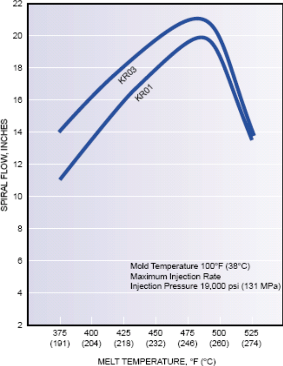
Figure 1 Spiral Flow as Function of Melt Temperature
